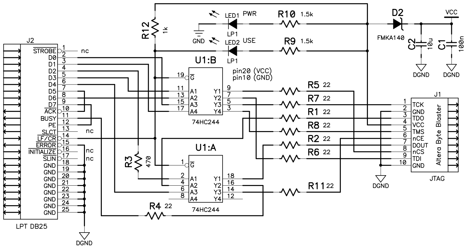
Pin connection to the JTAG (J1)
